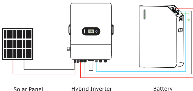
Figure 3-1 Single Battery System Connection Diagram
