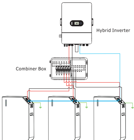
Figure 4-1 The parallel connection of three battery packs
