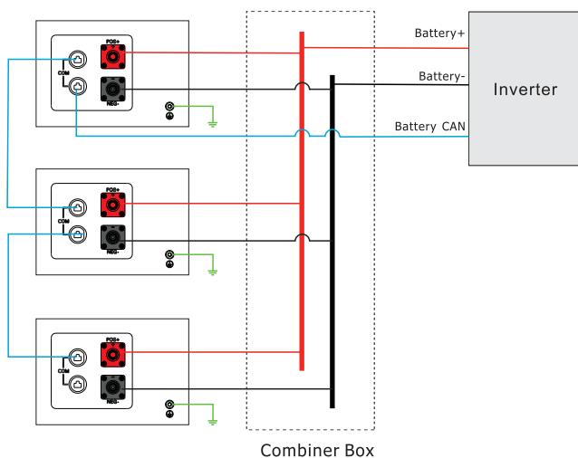
Figure 4-1 The parallel connection of three battery packs
